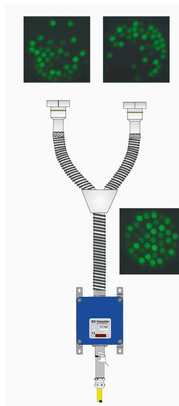
Merging of two flame signals to one flame scanners / CFC.
